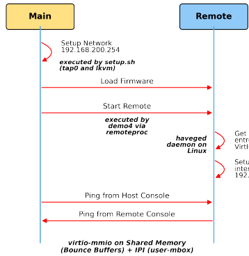
Fig. 3. Control flow diagram of the communication process
